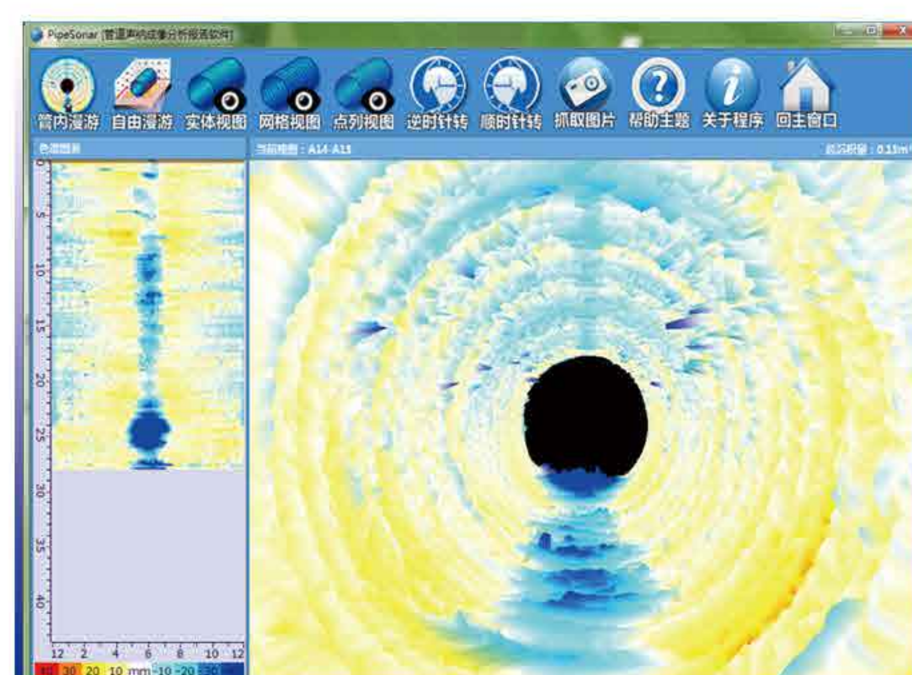
3D pipe rooming diagram
