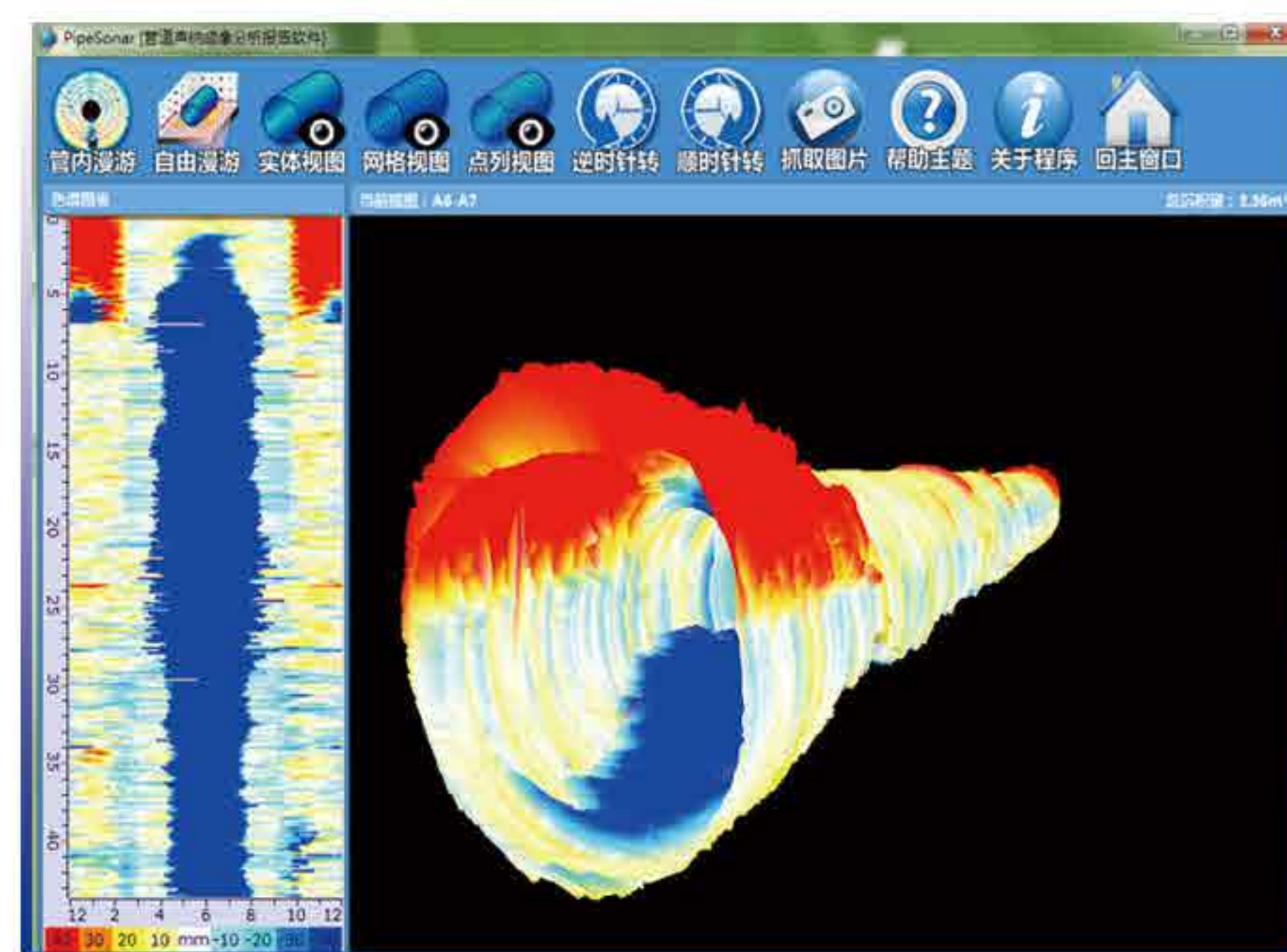
Profile diagram and 3d diagram of pipe
